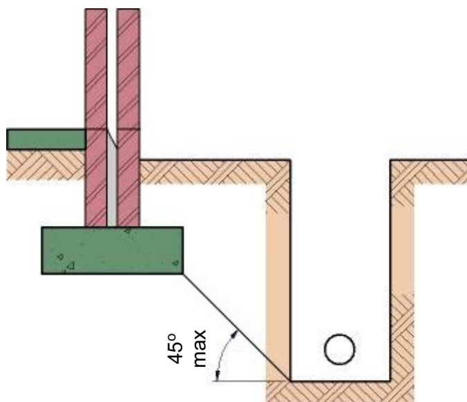
Position of drainage trench near foundation
